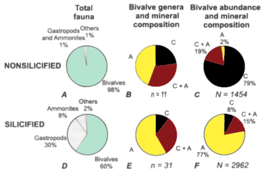
Figure 2. Pie diagrams for nonsilicified Porthkerry Formation faunas (A–C) and for silicified faunas (D–F), showing composition of total fauna (A, D), shell mineral composition for bivalve generic diversity (B, E; n = no. of genera) and for bivalve abundance (C, F; N = no. of individuals). Shell minerals: C—calcitic; C + A—biminerally; A—aragonitic.
