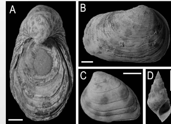
Figure 3. Molluscs from silicified fauna, showing fine preservation of shell features; scale bars represent 1 cm. Note beekitized patches on shell in A and C. A: Gryphaea arcuata , dorsal view. B: Pholadomya glabra , right valve. C: Cardinia listeri , left valve. D: Allocosmia .
