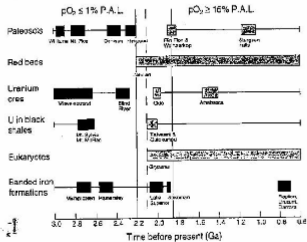
FIGURE 1. Summary of data bearing on the O_2 content of the Precambrian atmosphere.
