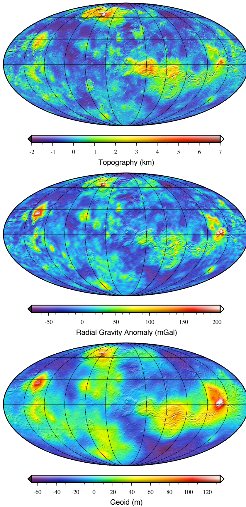
Figure 3. (top) Global topography of Venus derived from the 360 degree spherical harmonic model of Rappaport et al. (1999) referenced to geoid. (middle) Radial free-air gravity, evaluated at a radius of 6051 km, obtained after truncating the spherical harmonic coefficients of MGNP180U beyond degree 65. (bottom) First-order geoid obtained from the same coefficients as the radial gravity field. All images are in a Mollweide projection with a central meridian of 60° E longitude and are overlain by a gradient image derived from the topography model.
