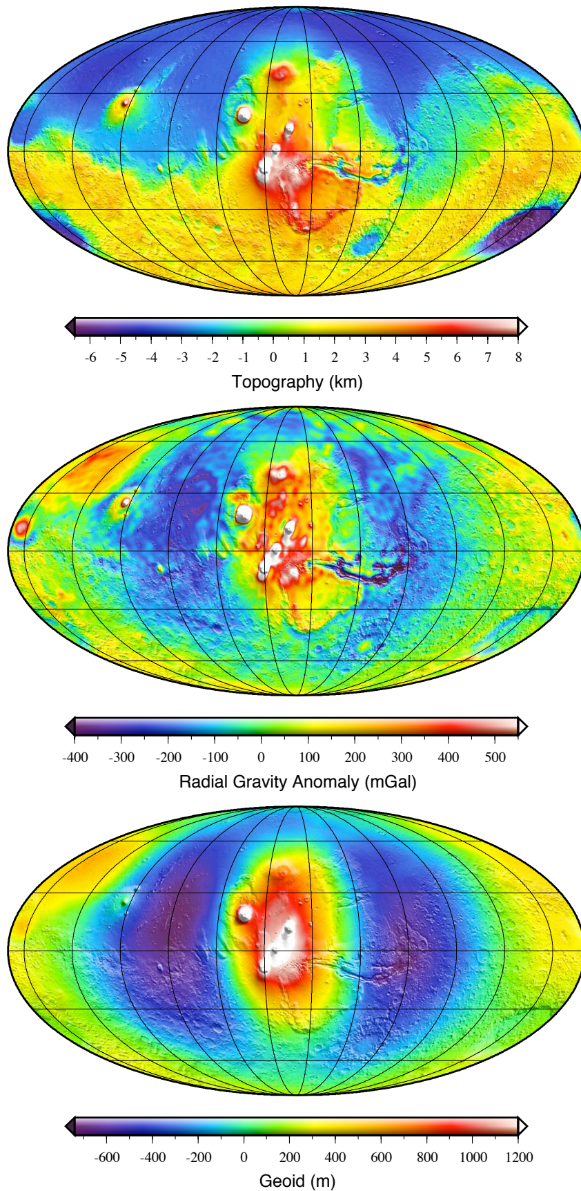
Figure 5. (top) Global topography of Mars (derived from the 90th degree spherical harmonic model Mars2000) referenced to the geoid calculated to second order accuracy. (middle) Radial free-air gravity, evaluated at a radius of 3396 km, obtained after truncating the spherical harmonic coefficients of JGM95J01 beyond degree 75 and setting the J_2 term to zero. (bottom) First-order geoid obtained from the same coefficients as the radial gravity field. All images are in a Mollweide projection with a central meridian of 100° W longitude and are overlain by a gradient image derived from the topography model.
