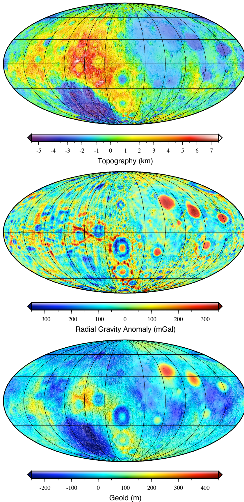
Figure 7. (top) Global topography of the Moon from the spherical harmonic model MoonUSGS359 referenced to the geoid which includes both the LP150Q gravitational model and rotational and tidal effects. (middle) Radial free-air gravity obtained from the model LP150Q evaluated at a radius of 1738 km after truncating the coefficients beyond degree 130 and setting the C_{2,0} and C_{2,2} terms equal to zero. (bottom) First-order geoid obtained from the same coefficients as the radial gravity field. All images are in a Mollweide projection with a central meridian of 90^\circ W longitude and are overlain by the shaded relief map of Rosiek and Aeschliman (2001). The near- and farside hemispheres are on the right and left halves of these images, respectively.
