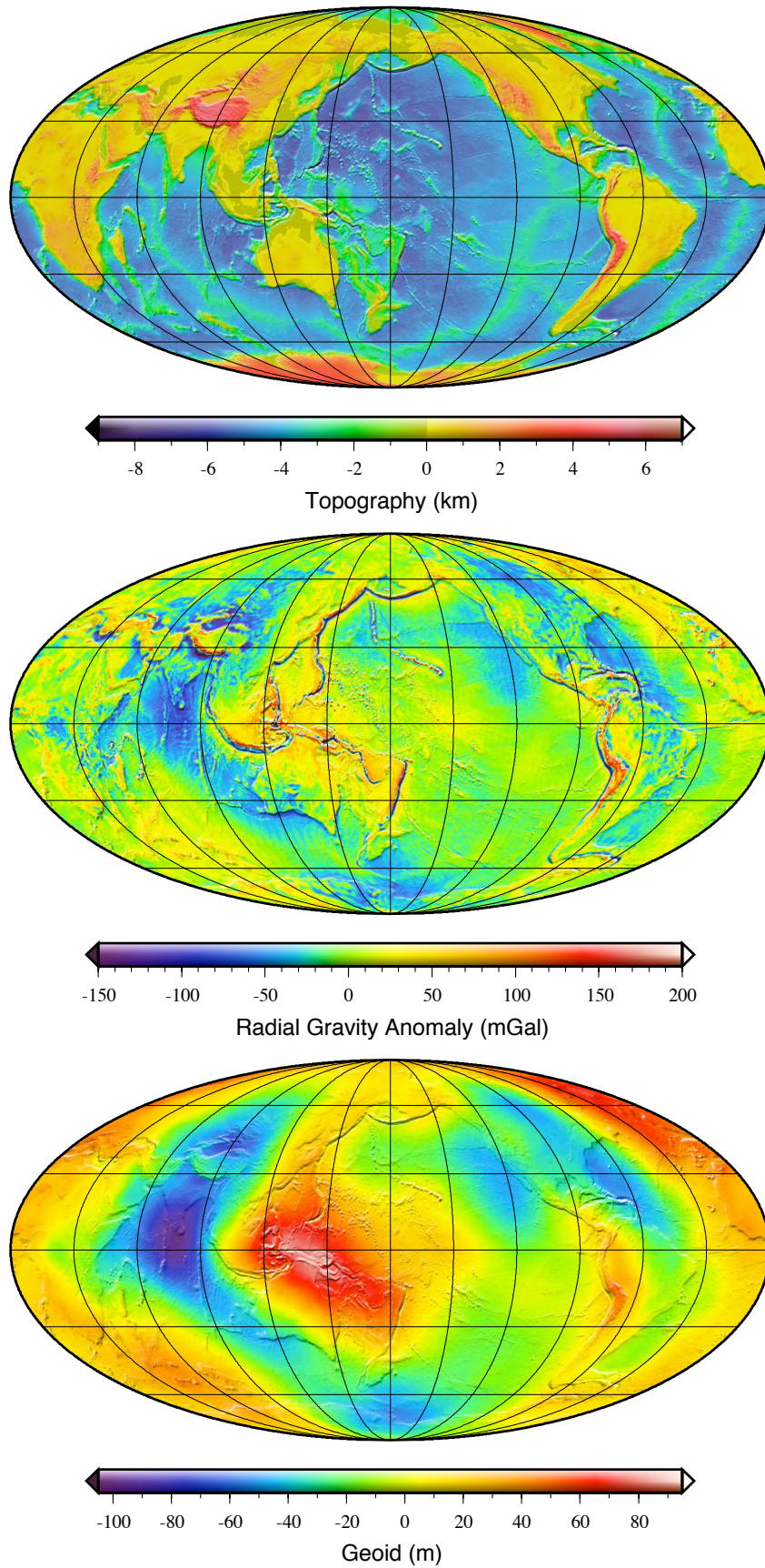
Figure 1. (top) Global topography and bathymetry of the Earth, referenced to mean sea level, of the model SRTM30_PLUS. (middle) Radial free-air gravity from EIGEN-CG03C, obtained after setting the zonal degree-2 term equal to zero, evaluated at a radius of 6378.1 km. (bottom) First-order geoid obtained from the same coefficients as the radial gravity field. All images are in a Mollweide projection with a central meridian of 180° W longitude and are overlain by a gradient image derived from the topography model.
