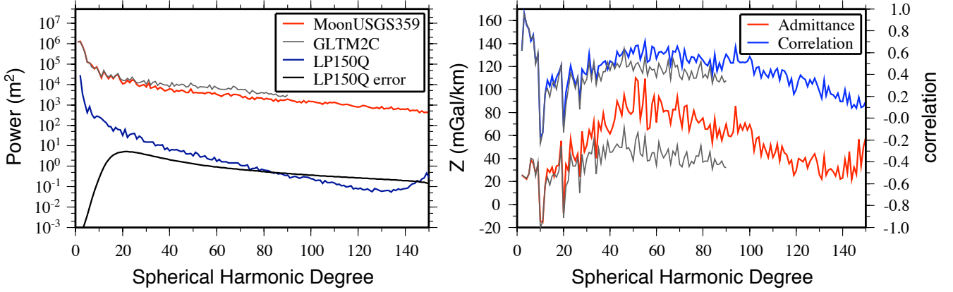
Figure 8. Power and cross-power spectra of the Moon's gravity and topography. (left) Power spectra of the topographic models MoonUSGS359 and GLTM2C, and the LP150Q geoid and error. (right) Gravitational admittance and correlation spectra using MoonUSGS359 (color) and GLTM2C (gray).
