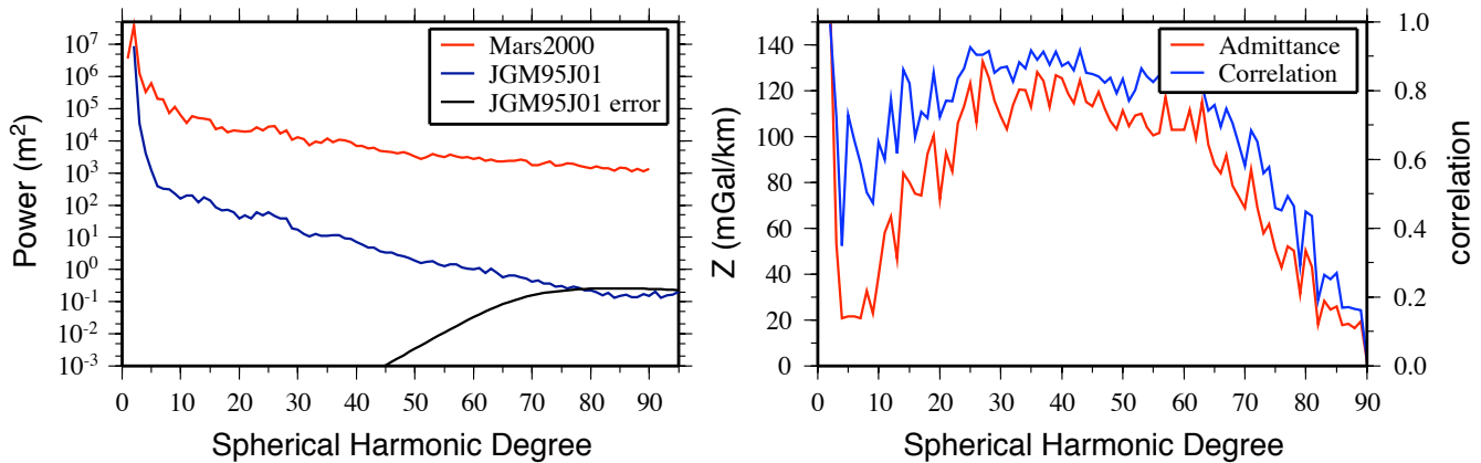
Figure 6. Power and cross-power spectra of the gravity and topography of Mars. (left) Power spectra of the topography (Mars2000), geoid (JGM95J01), and geoid error. (right) Gravitational admittance and correlation spectra of the two fields.
