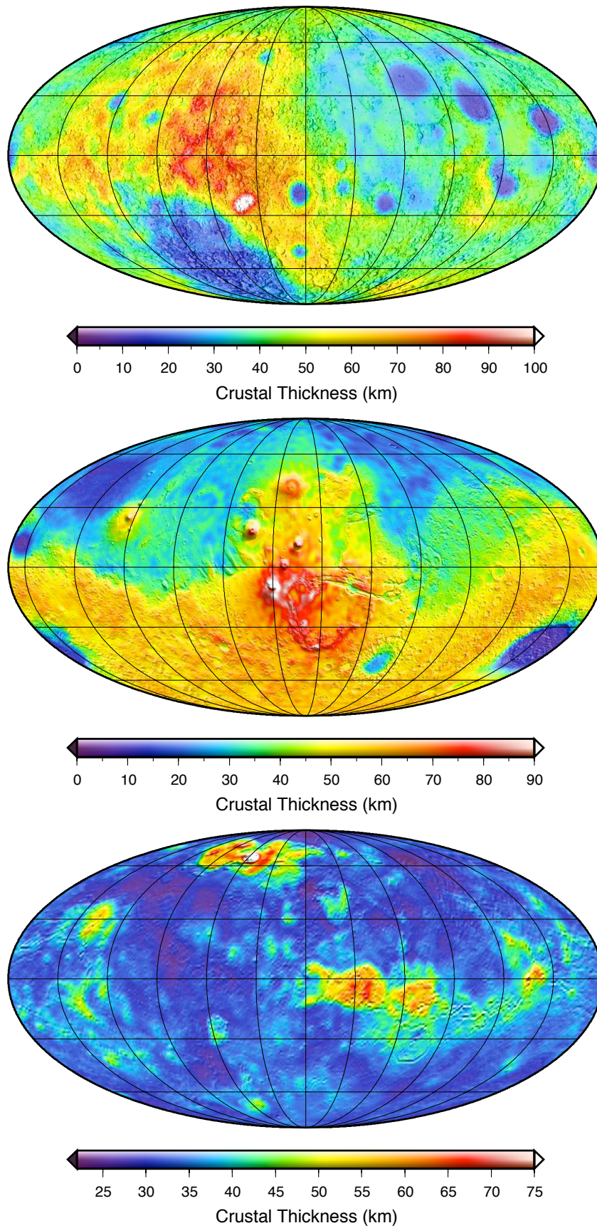
Figure 10. Crustal thickness models for the Moon (top), Mars (middle), and Venus (bottom). See sections 5 and 8 for details.
