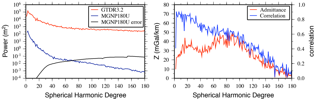
Figure 4. Power and cross-power spectra of the gravity and topography of Venus. (left) Power spectra of the topography (GTDR3.2), geoid (MGNP180U), and geoid error. (right) Gravitational admittance and correlation spectra of the two fields.
