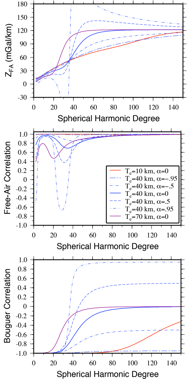
Figure 11. (top) Free-air admittance, (middle) free-air correlation, and (bottom) Bouguer correlation, for a flexural model with equal magnitudes of applied surface and subsurface loads. Model parameters correspond to the planet Mars, with T_c = z = 50 km, \rho_c = 2900 kg m ^{-3} , \rho_m = 3500 kg m ^{-3} , and E = 10^{11} Pa. Solid lines correspond to the case where the applied surface and subsurface loads have random phases (i.e., \alpha = 0 ), and the dashed lines correspond to the case where these loads are partially correlated.
