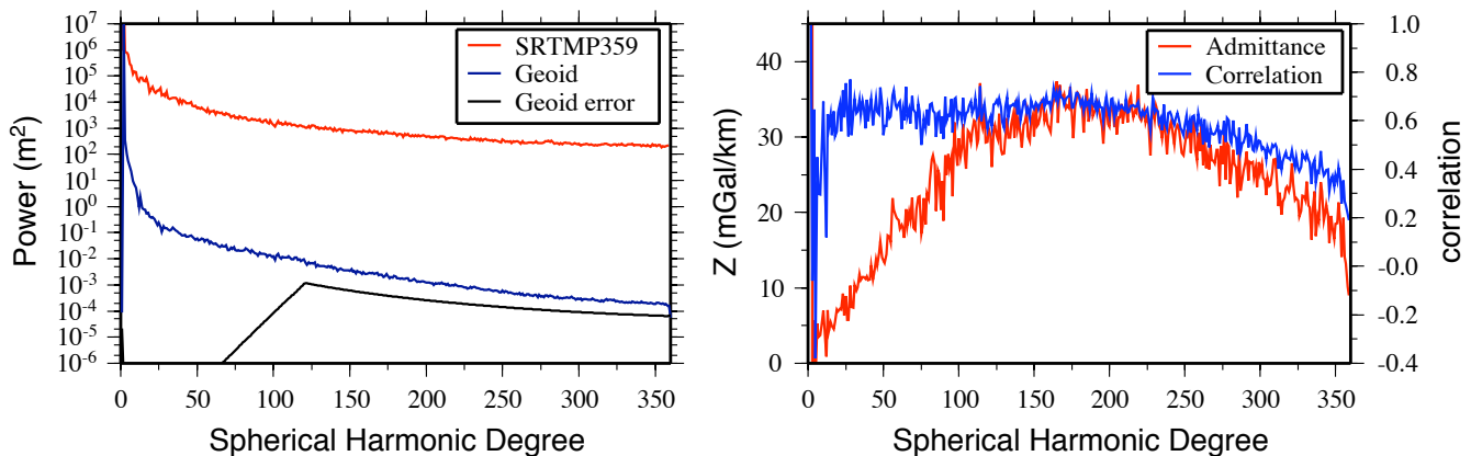
Figure 2. Power and cross-power spectra of the Earth's gravity and topography. (left) Power spectra of the topography (SRTMP359), geoid (EIGEN-CG03C), and calibrated geoid error. (right) Gravitational admittance and correlation spectra of the two fields.
