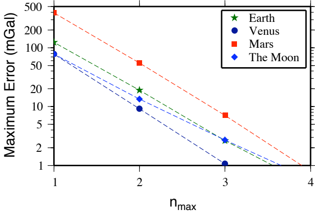
Figure 9. Maximum error associated with the Bouguer correction as a function of the order n_{\max} used in eq. 28. The Bouguer correction is here defined as the radial gravitational attraction resulting from surface relief with respect to the mean planetary radius. The true value was approximated by n_{\max} = 10 , the crustal density was assumed to be 2900 \text{ kg m}^{-3} , and the radial gravity anomaly was evaluated at the maximum elevation of the planet.
